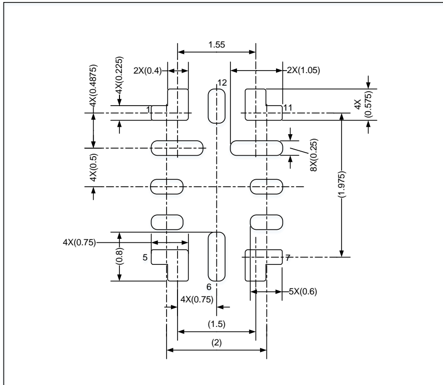
Figure 9-2 QFN12 recommend Footprint
