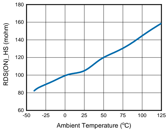
Figure 3. High-Side RDS(ON) vs. Temperature
