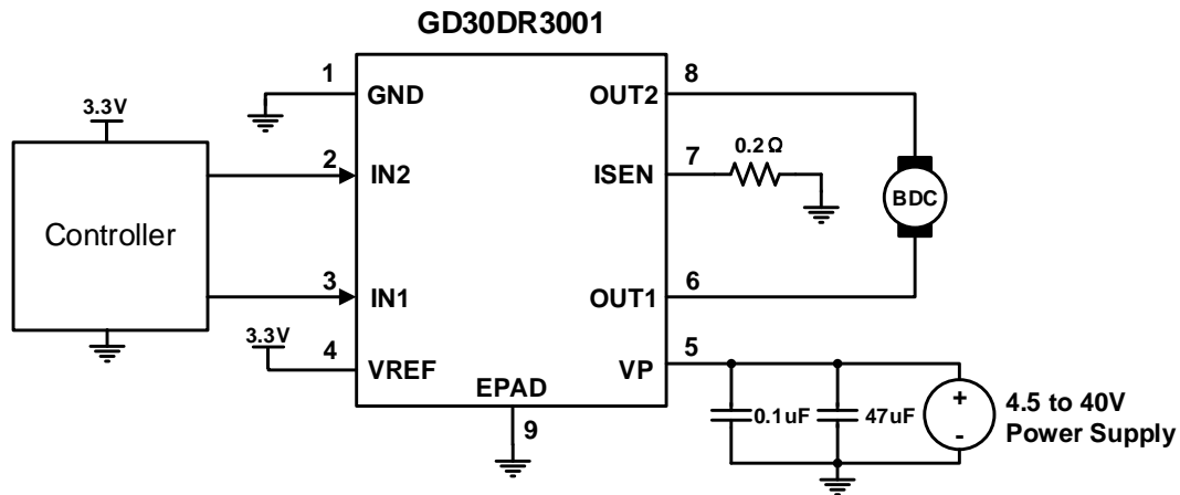
Figure 9. Schematic of GD30DR3001 Application
