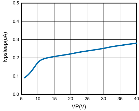
Figure 1. Sleep Current vs. Input Voltage
