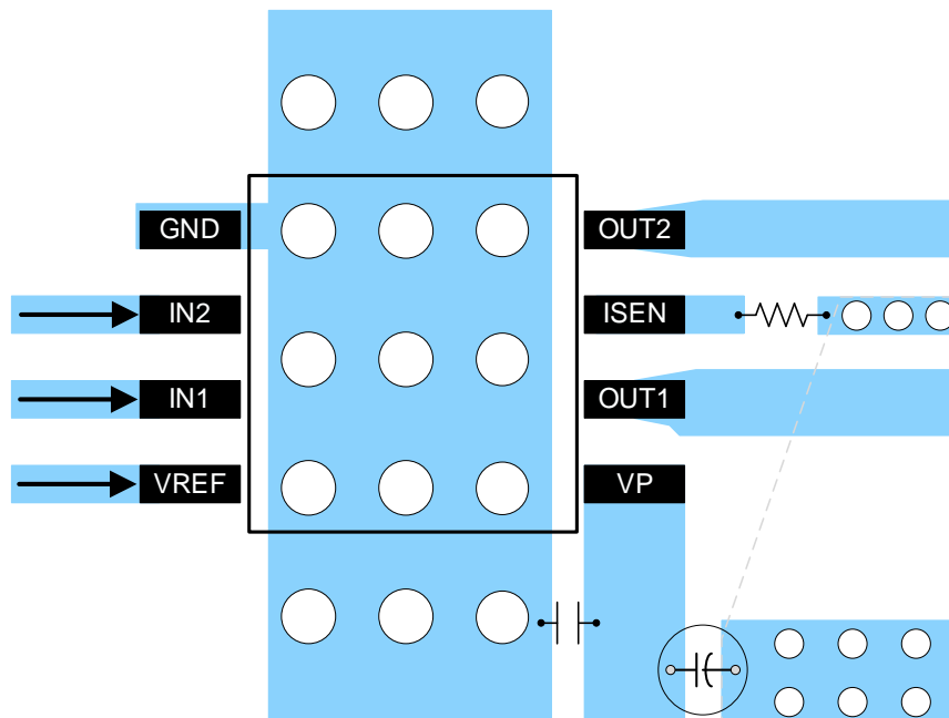
Figure 17. Simplified Layout Example
