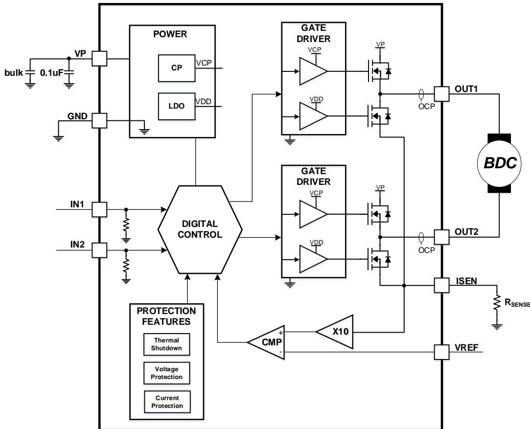
Figure 6. GD30DR3001 Functional Block Diagram
