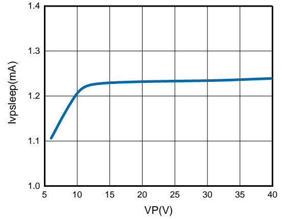
Figure 2. Active Current vs. Input Voltage
