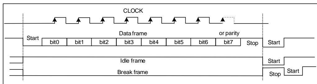
Figure 20-2. USART character frame (8 bits data and 1 stop bit)
