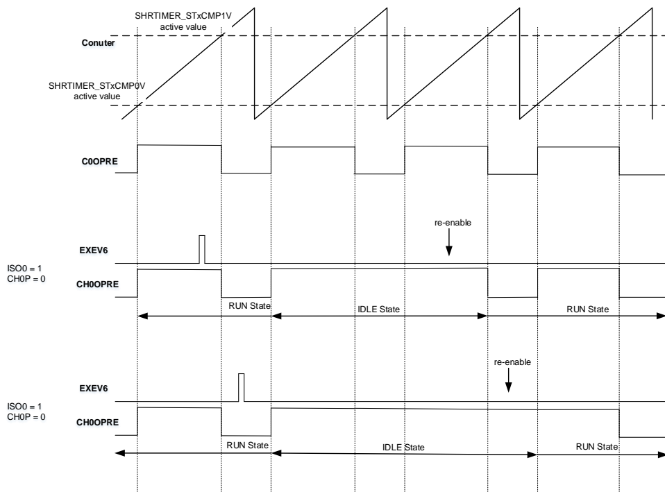
Figure 19-31. ISO0 = 1 and CHOP = 0 in delayed IDLE
