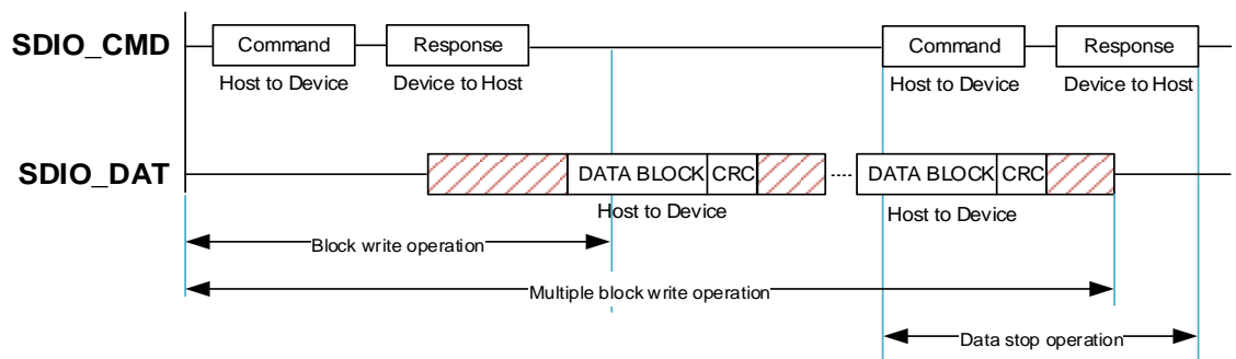
Figure 24-3. SDIO multiple blocks write operation
