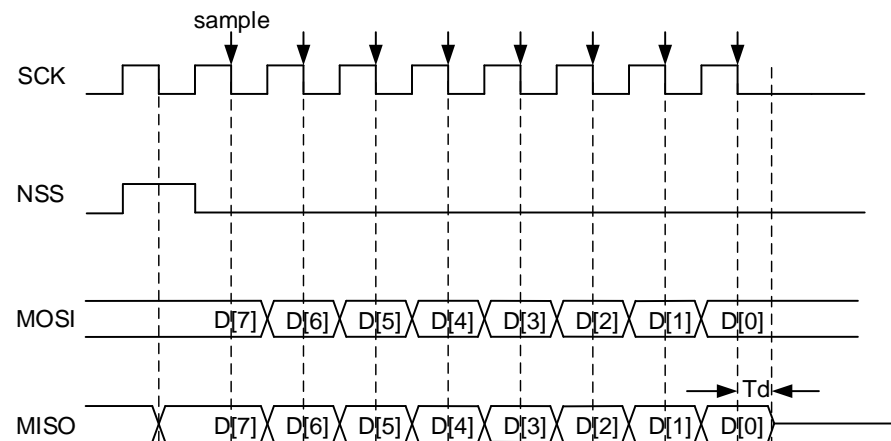
Figure 22-10. Timing diagram of TI slave mode
