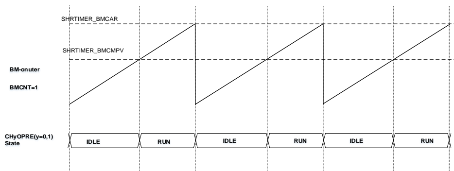
Figure 19-39. Bunch mode timing chart
