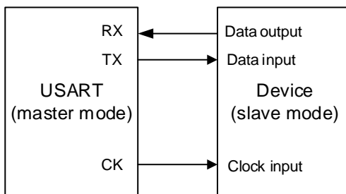
Figure 20-11. Example of USART in synchronous mode
