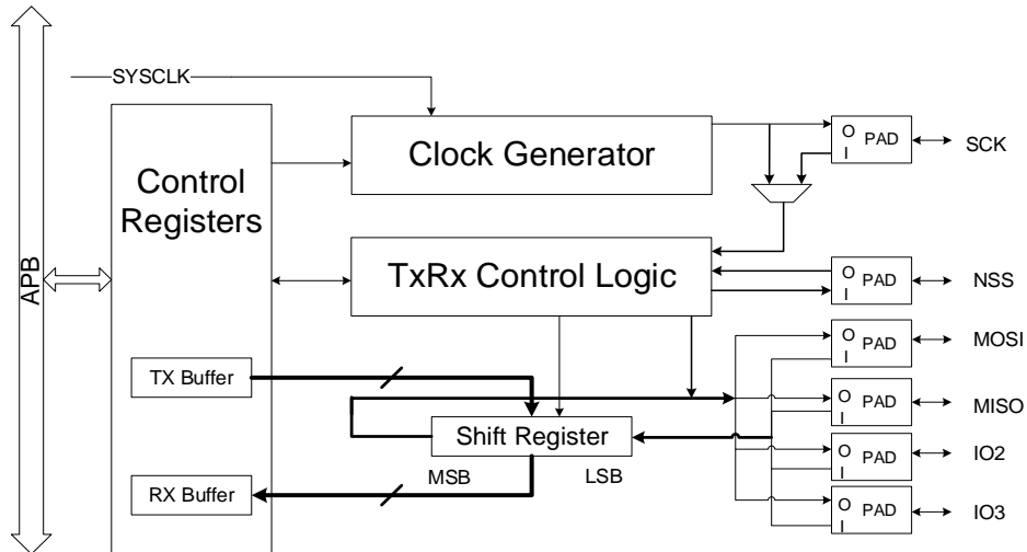
Figure 22-1. Block diagram of SPI
