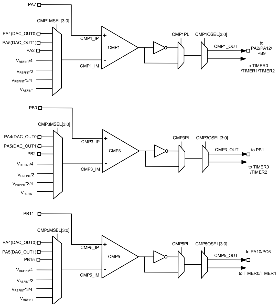
Figure 15-1. CMP block diagram of GD32E50x series
