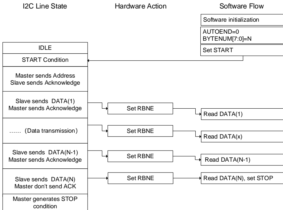
Figure 21-33. Programming model for master receiving (N<=255)
