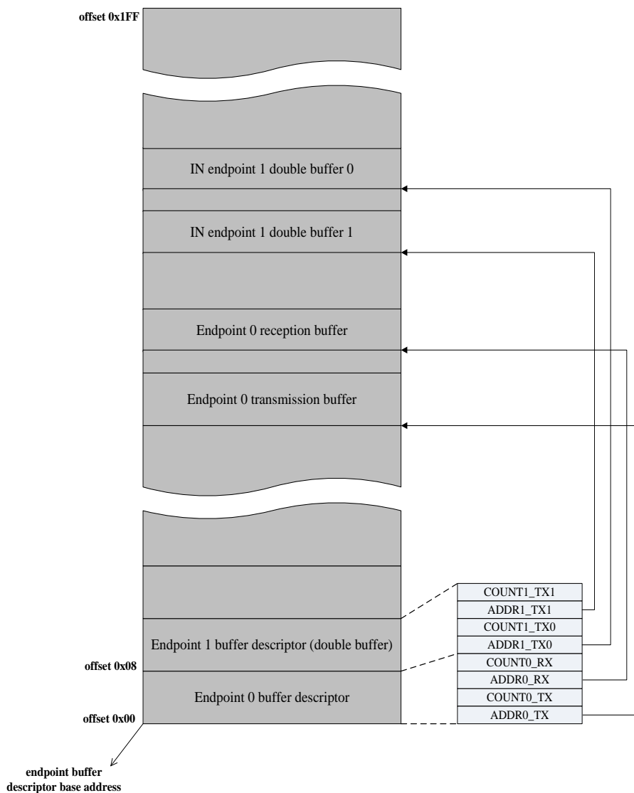
Figure 28-2. An example with buffer descriptor table usage (USB_D_BADDR = 0)
