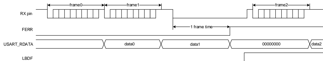
Figure 20-23. Break frame occurs during idle state
