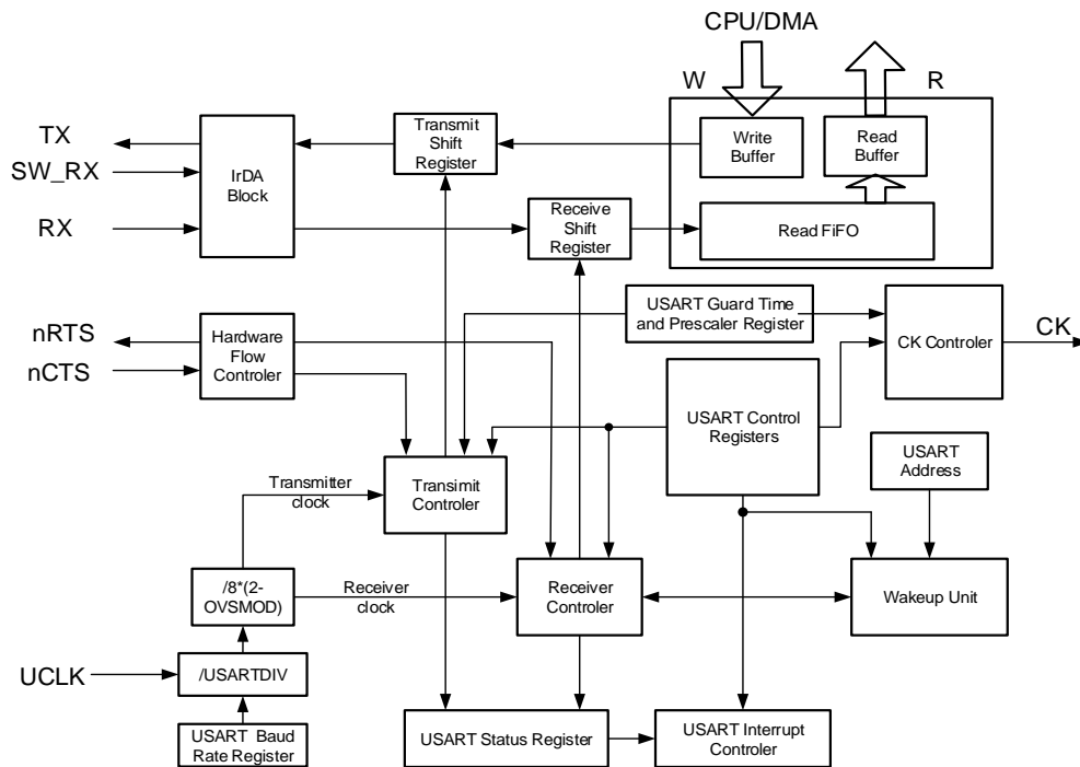
Figure 20-17. USART module block diagram
