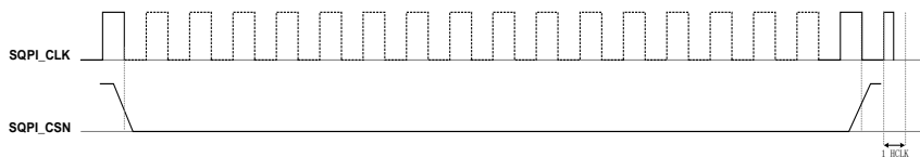
Figure 23-4. SQPI_CLK Example
