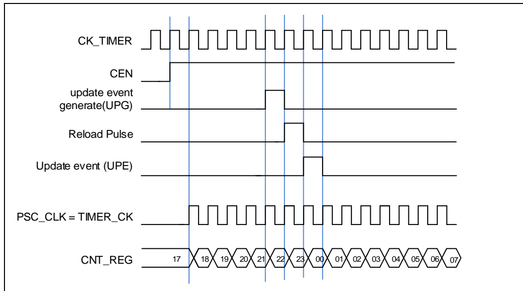
Figure 18-31. Timing chart of internal clock divided by 1
