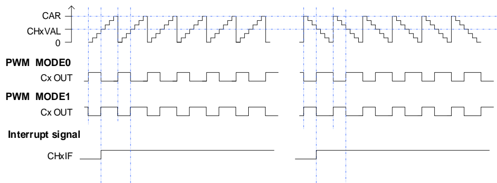
Figure 18-41. Timing chart of EAPWM
