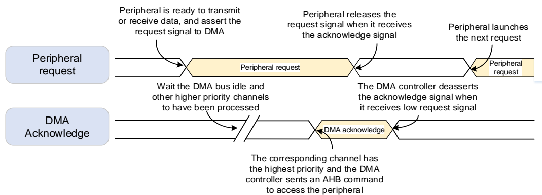
Figure 11-2. Handshake mechanism
