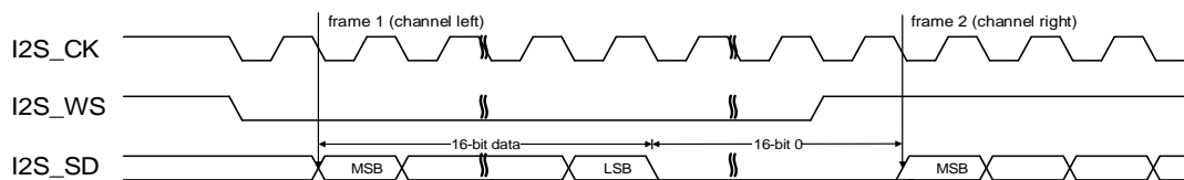
Figure 22-22. I2S Phillips standard timing diagram (DTLEN=00, CHLEN=1, CKPL=1)
