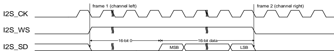
Figure 22-33. LSB justified standard timing diagram (DTLEN=00, CHLEN=1, CKPL=0)
