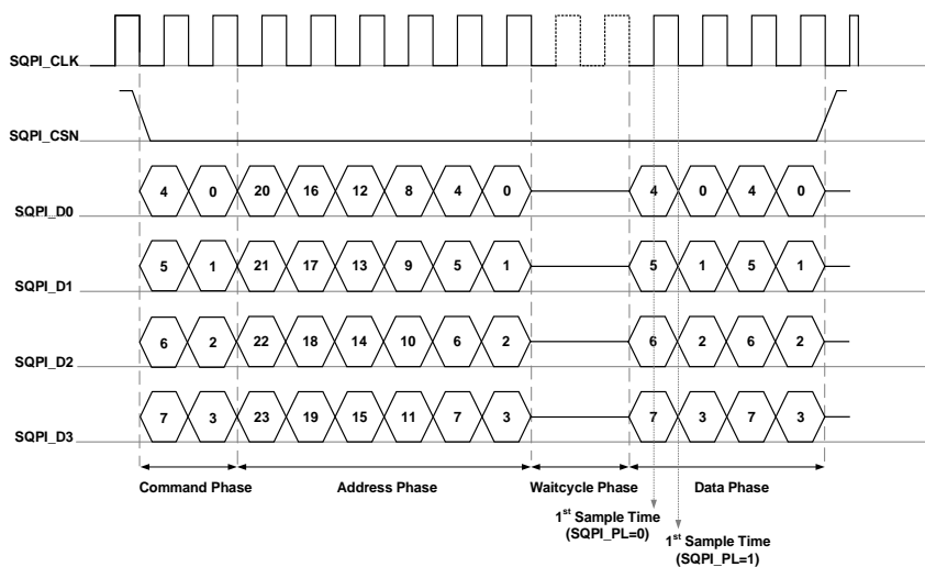
Figure 23-1. SQPI_PL Example
