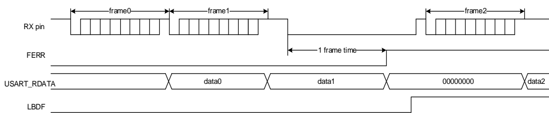
Figure 20-9. Break frame occurs during idle state
