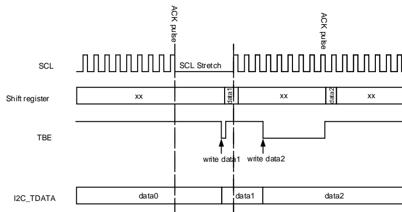
Figure 21-24. Data transmission
