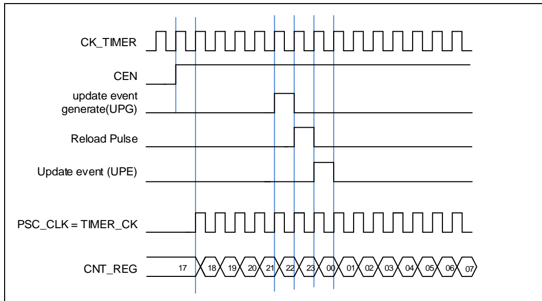
Figure 18-47. Timing chart of internal clock divided by 1
