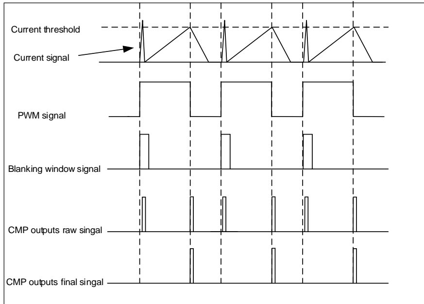
Figure 15-2. The CMP outputs signal blanking
