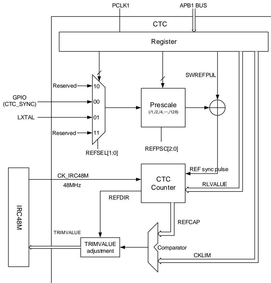
Figure 6-1. CTC overview
