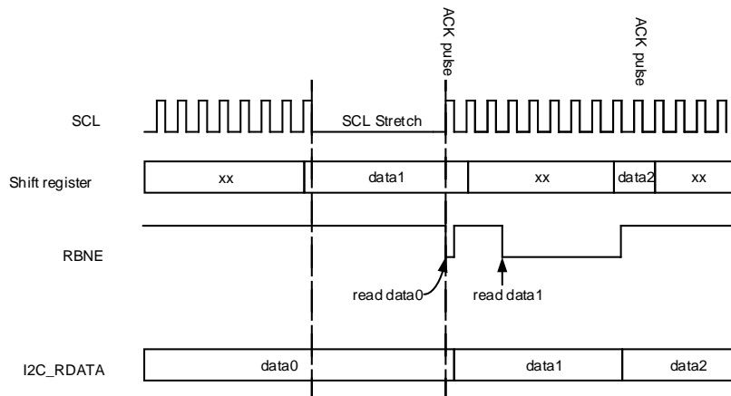
Figure 21-25. Data reception
