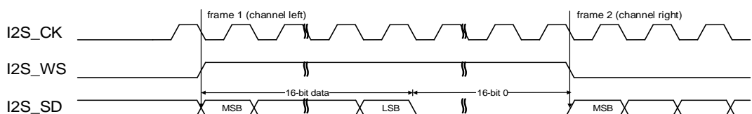
Figure 22-29. MSB justified standard timing diagram (DTLEN=00, CHLEN=1, CKPL=0)
