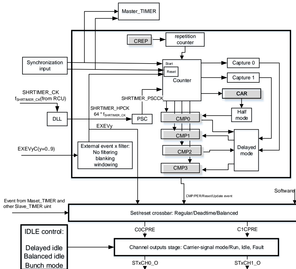
Figure 19-10. Slave_TIMERx diagram
