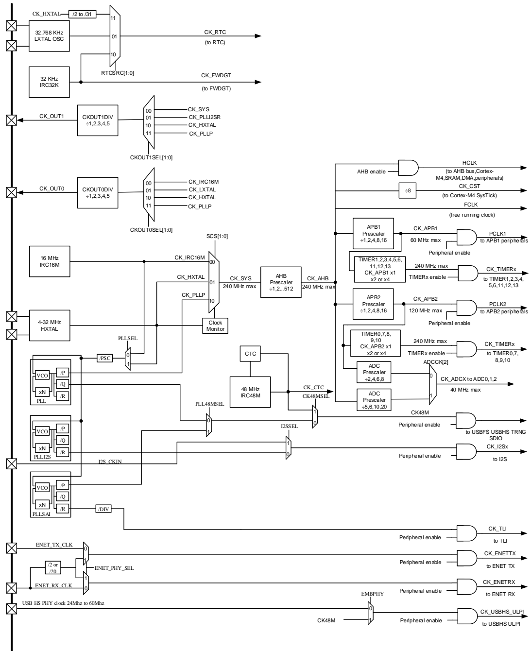
Figure 4-2. Clock tree
