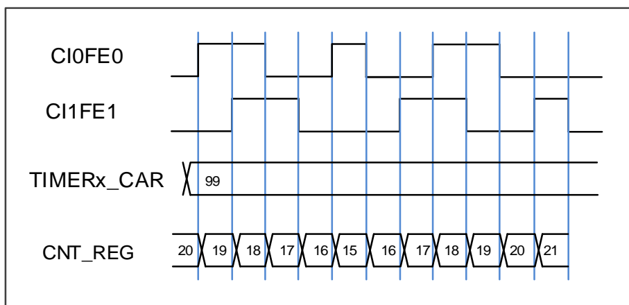
Figure 18-19. Counter behavior with CI0FE0 polarity inverted in mode 2
