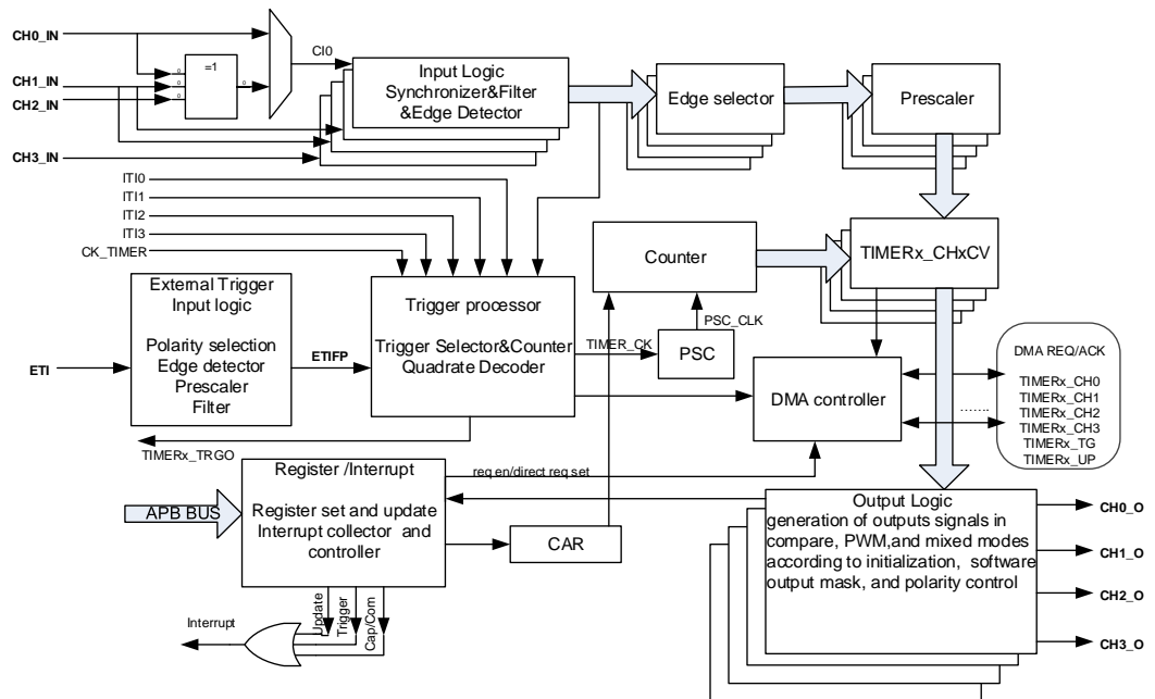
Figure 18-28. General Level 0 timer block diagram
