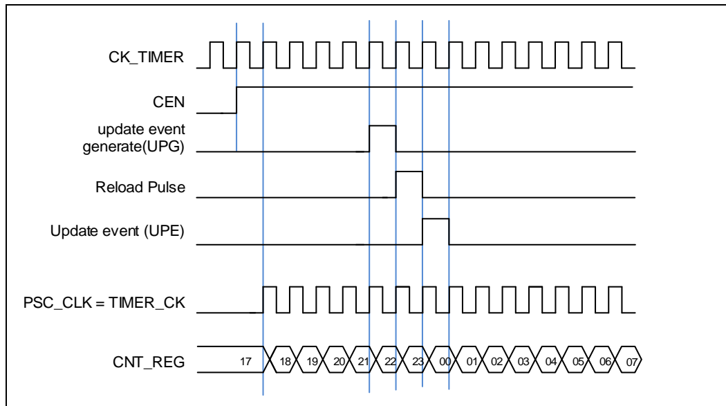
Figure 18-29. Timing chart of internal clock divided by 1
