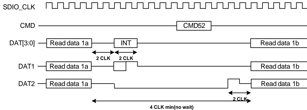
Figure 24-13. Read wait operation using SDIO_DAT[2]
