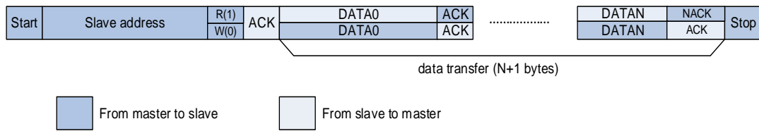
Figure 20-6. I2C communication flow with 7-bit address
