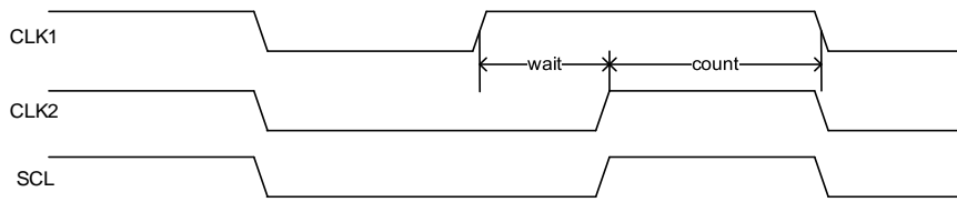
Figure 20-4. Clock synchronization
