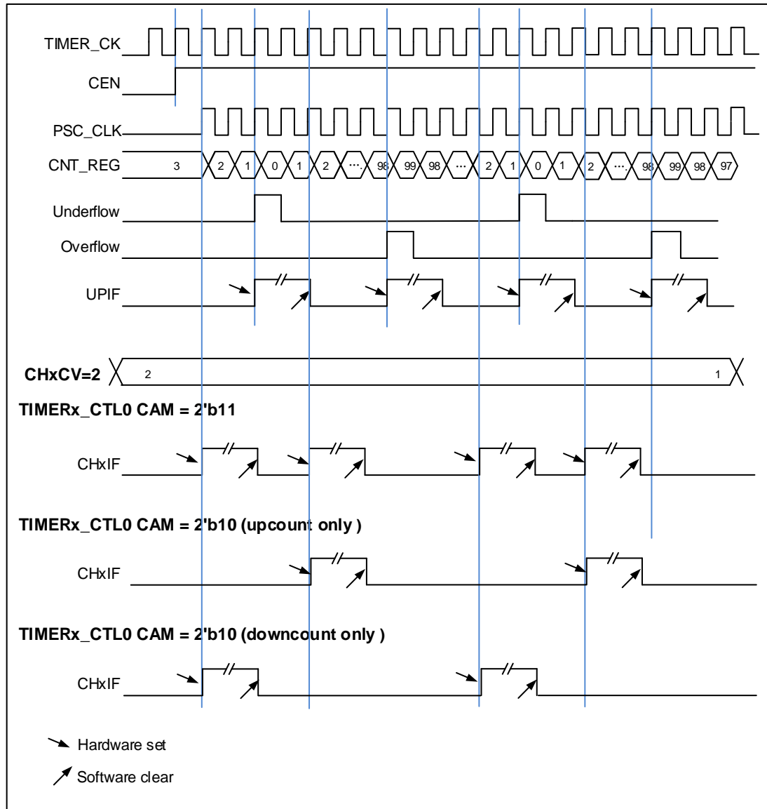
Figure 18-35. Timing chart of center-aligned counting mode
