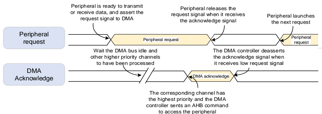
Figure 10-3. Handshake mechanism
