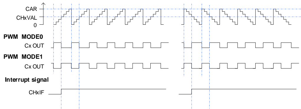
Figure 18-39. CAPWM timechart
