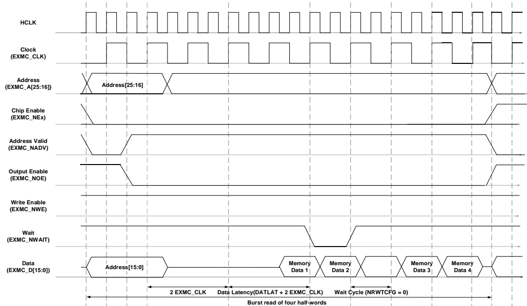
Figure 25-22. Read timing of synchronous multiplexed burst mode
